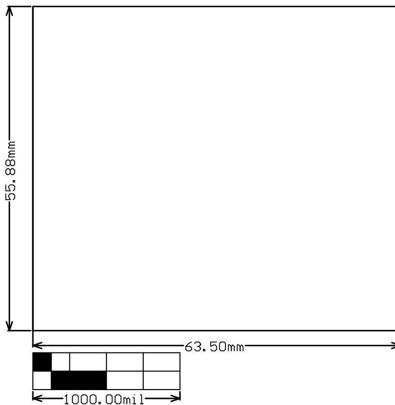
Figure 16. Board Dimensions
