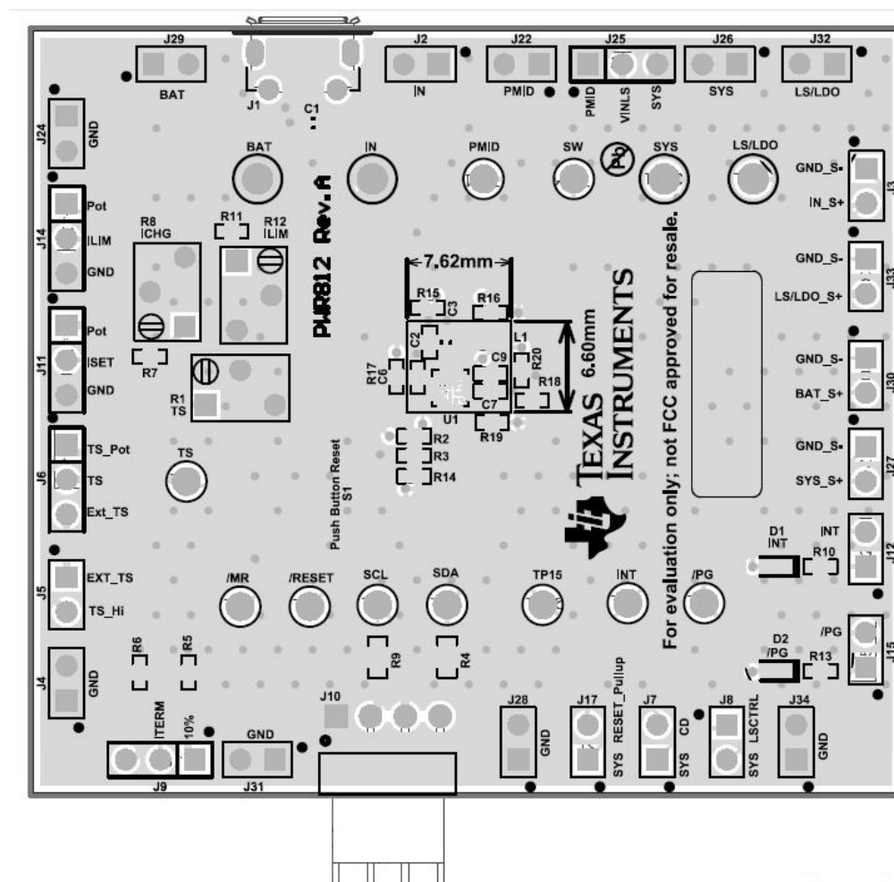
Figure 17. PWR812 Composite Layout
