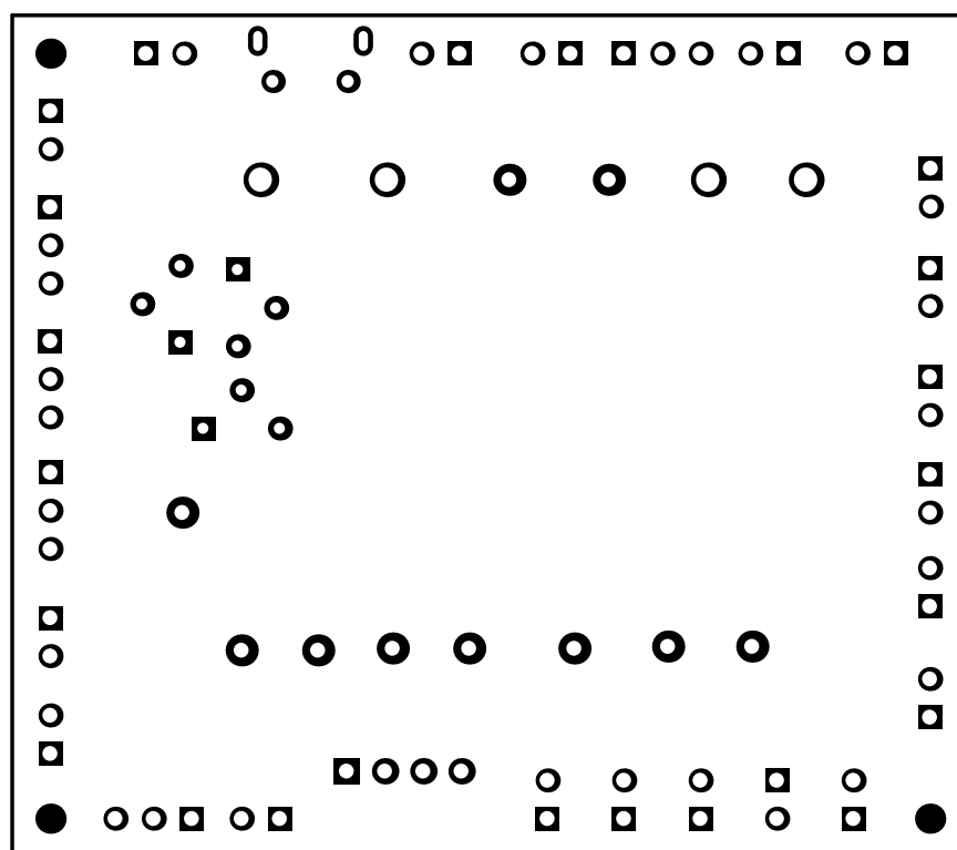
Figure 14. Bottom Overlay
